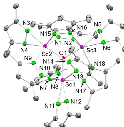
Fig. 6 Crystal structure of [\text{Sc}_3\text{O}(\text{pz}^{\text{Me}_3})_7(\text{Hpz}^{\text{Me}_3})_2] ( 8 ). Ellipsoids are set at the 50% probability level. Hydrogen atoms are omitted for clarity. See ESI† for selected interatomic distances and angles.
