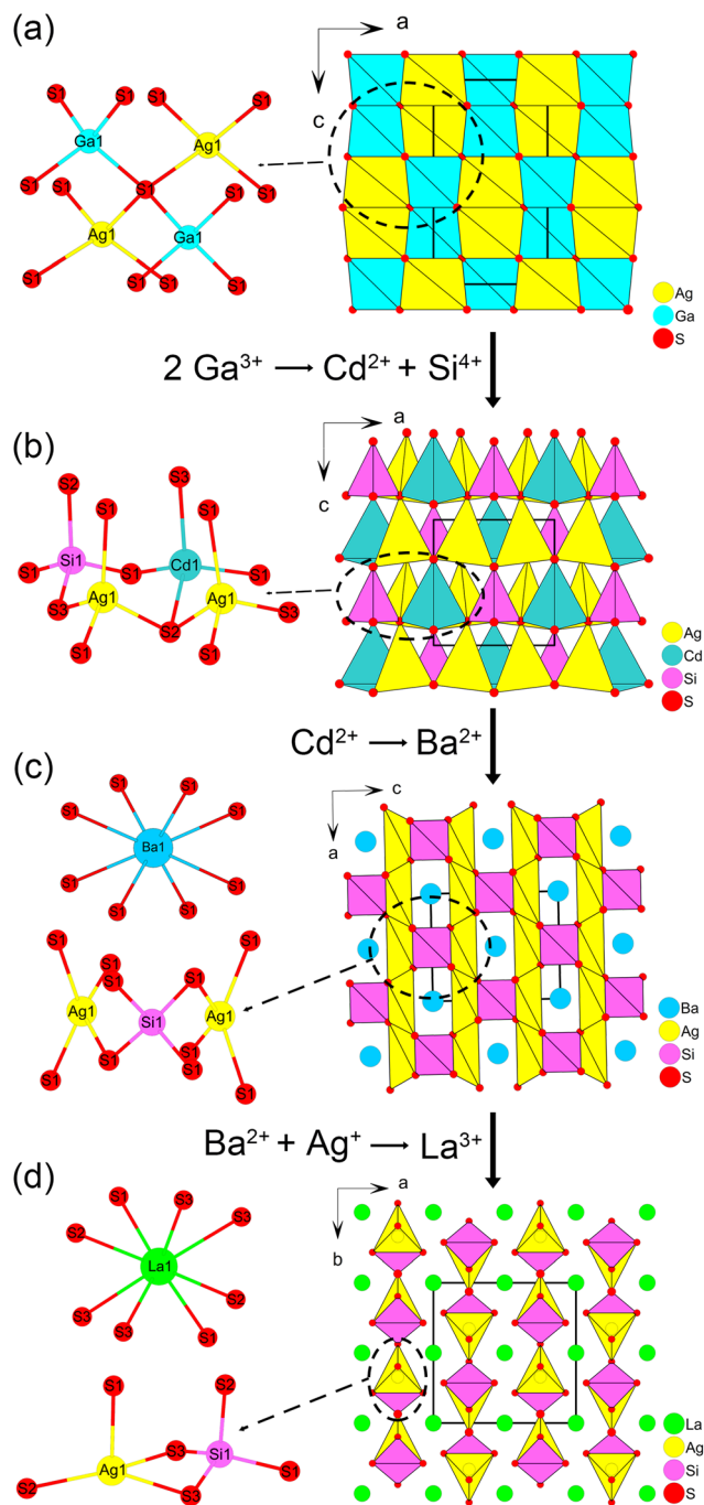
Fig. 1 Vertex-shared \text{Ag}_4\text{S}_4 , \text{Ga}_4\text{S}_4 tetrahedra; three-dimensional diamond-like \text{AgGa}_2\text{S}_4 crystal structures (a); vertex-shared \text{Ag}_4\text{S}_4 , \text{Cd}_4\text{S}_4 and \text{Si}_4\text{S}_4 tetrahedra; three-dimensional tetrahedra closed-packed \text{AgCdSi}_4 crystal structures (b); coordination environment of \text{Ba}^{2+} ; vertex-shared \text{Ag}_4\text{S}_4 and \text{Si}_4\text{S}_4 tetrahedra; three-dimensional tunnel structure of \text{BaAg}_2\text{Si}_4 (c); coordination environment of \text{La}^{3+} ; edge-shared \text{Ag}_4\text{S}_4 and \text{Si}_4\text{S}_4 tetrahedra; crystal structure of \text{LaAgSi}_4 composed of [\text{AgSi}_4\text{S}_4]^{5-} layers (d).
