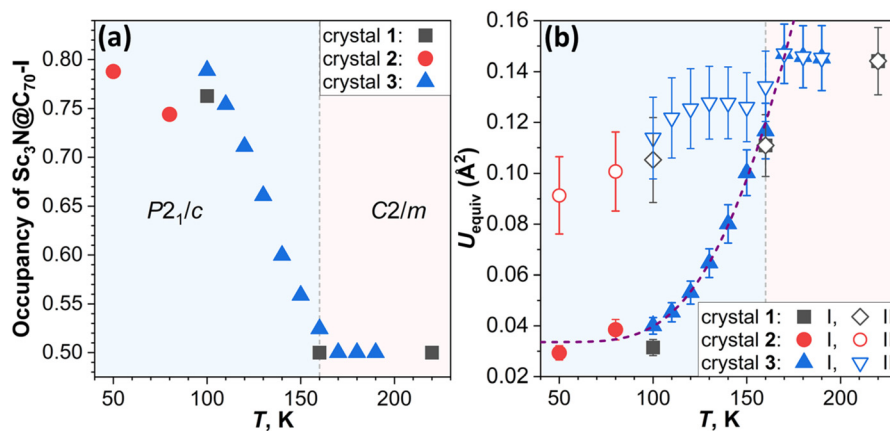
Fig. 2 (a) The site occupancy of Sc 3 N@C 70 orientation I vs. temperature. (b) Temperature dependence of the average equivalent atom displacement parameter ( U_{\text{equiv}} ) of the carbon cage in two orientations of the Sc 3 N@C 70 molecule (I and II), error bars denote standard deviations within the sets of 70 carbons; dashed purple line is the fit of the data for orientation I in crystal 3 between 100 and 170 K by a function a + b\text{cth}(\hbar\nu/2kT) .
