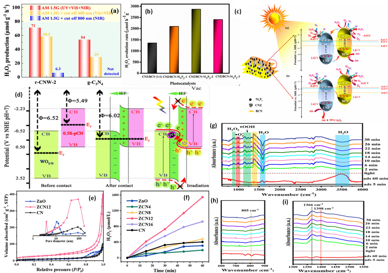
Fig. 28 (a) \text{H}_2\text{O}_2 production by g-C 3 N 4 and r-CNW-2 under simulated solar, visible, and NIR light illumination for 1 h. The figures are adapted with permission from ref. 208. Copyright 2023, Elsevier. (b) \text{H}_2\text{O}_2 generation rates of CNZ/BCN(1:1) and CNZ/BCN-Ni x P y -x samples. (c) Diagram of photocatalytic \text{H}_2\text{O}_2 and \text{H}_2 formation mechanisms by the CNZ/BCN-Ni x P y -2 composite. The figures are adapted with permission from ref. 209. Copyright 2023, ACS. (d) Diagrams of the S-scheme heterojunction between WO 3 and 0.5S-pCN before and after contact, showing IEF formation and band bending. The figures are adapted with permission from ref. 212. Copyright 2021, Elsevier. (e) N 2 adsorption-desorption isotherms and pore size distribution profiles. (f) \text{H}_2\text{O}_2 photocatalysis by samples under UV-vis light. The figures are adapted with permission from ref. 151. Copyright 2021, ACS. In situ DRIFTS spectra of SCN/T9 during \text{H}_2\text{O}_2 generation at (g) 600–4000 \text{cm}^{-1} , (h) 600–900 \text{cm}^{-1} , and (i) 1300–1550 \text{cm}^{-1} . The figures are adapted with permission from ref. 213. Copyright 2023, Elsevier.
