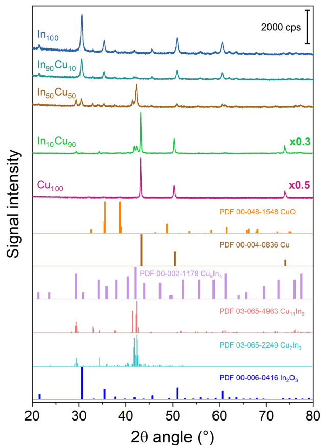
Fig. 6 XRD diffractograms of the spent TC samples. For the sake of clarity, a diffractogram with multiplicative values has the measured intensity multiplied by that factor.
