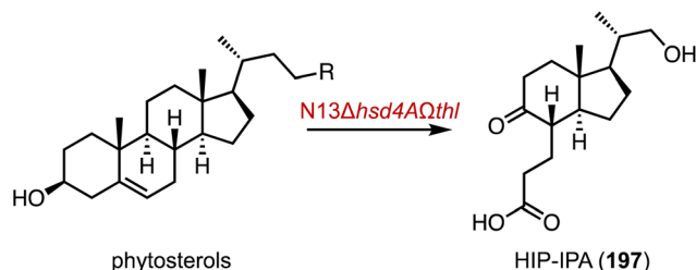
Fig. 32 Biotransformation of phytosterols into 197.
