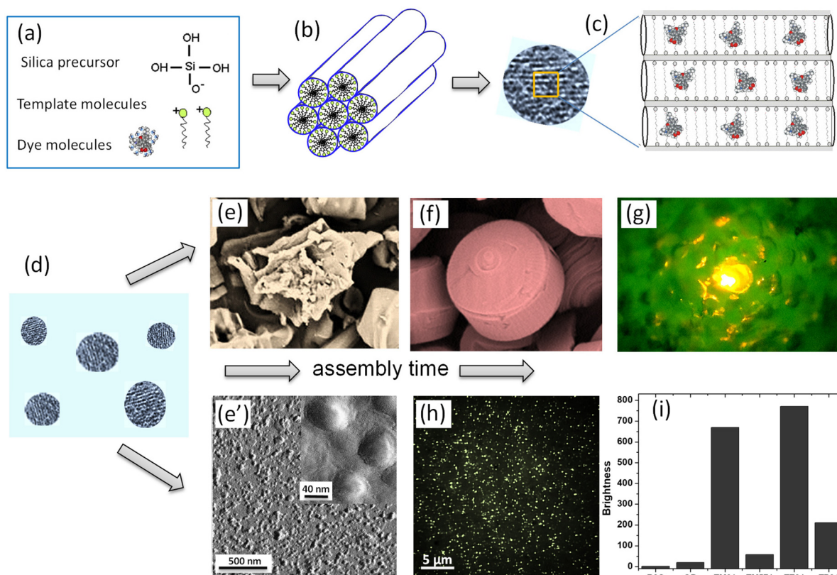
Fig. 1 A schematic of the mechanism of self-assembly of ultrabright mesoporous silica particles (UMSP). (a) The building blocks of the particles: template cationic surfactant molecules, which will form liquid crystals; a mineralizable inorganic anion, deprotonated silicate; and dye molecules. (b) Deprotonated silicate condenses on the surface of the nematic liquid crystals created by the template molecules. (c) Small nematic crystals are fused into silica mesoporous structures, "seed" particles, which carry fluorescent dye molecules encapsulated inside the cylindrical channels of the particles. (d) Initially sticky and not fully polymerized seed particles of 10–20 nm in size will now be the building blocks for both nano and micron size UMSP. (e) The seeds assemble into larger micron-size aggregates if allowed to stay in the synthesizing bath. (f) The micron-size aggregates have further been developed into mesoporous silica shapes with well-aligned cylindrical mesochannels. (g) An example of an ultrabright fluorescent discoid illuminating the landscape of surrounding polymer. (e') When suppressing the aggregation of seed particles, the seeds shown in panel (d) will be assembled and polymerized as separate nanoparticles. (h) A fluorescent image of the obtained nano-UMSP. (i) Relative fluorescent brightness of different nano-UMSP (TM91 is 40 nm, TM571 is 23 nm, TE91 is 52 nm, and TP91 is 45 nm (ref. 13)) versus single R6G molecule, ~30 nm water-dispersible (coated for protection and water "solubility" 60 ) CdSe/ZnS quantum dot with green fluorescence. [Compiled using images taken from ref. 18, 30, 37 and 61. Reproduced from ref. 18 with permission from John Wiley and Sons, copyright 2008; Reproduced from ref. 30 with permission from RCS, copyright 2021; Reproduced from ref. 37 with permission from RCS, copyright 2017; Reproduced from ref. 61 with permission from John Wiley and Sons, copyright 2010].
