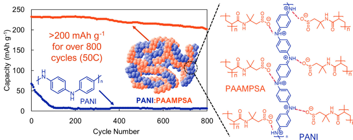
Fig. 11 Cycling of a pernigraline-polyaniline with a polyacid stabilizer (PANI:PAAMPSA) (orange) compared to pure polyaniline (PANI) (blue) at a 50C rate. Adapted with permissions from ref. 57. Copyright © 2013 Royal Society of Chemistry.
