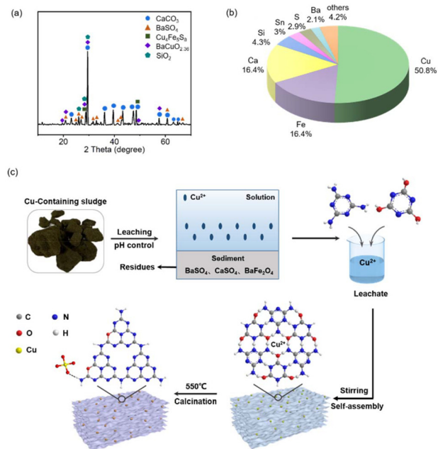
Fig. 1 (a) XRD pattern of the sludge. (b) Pie chart of the elemental distribution of the sludge. (c) Schematic illustration of the synthetic process of CuO/C 3 N 4 .
