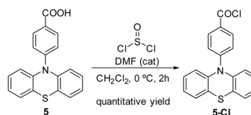
Scheme 3 Synthesis of acid chloride 5-Cl .
