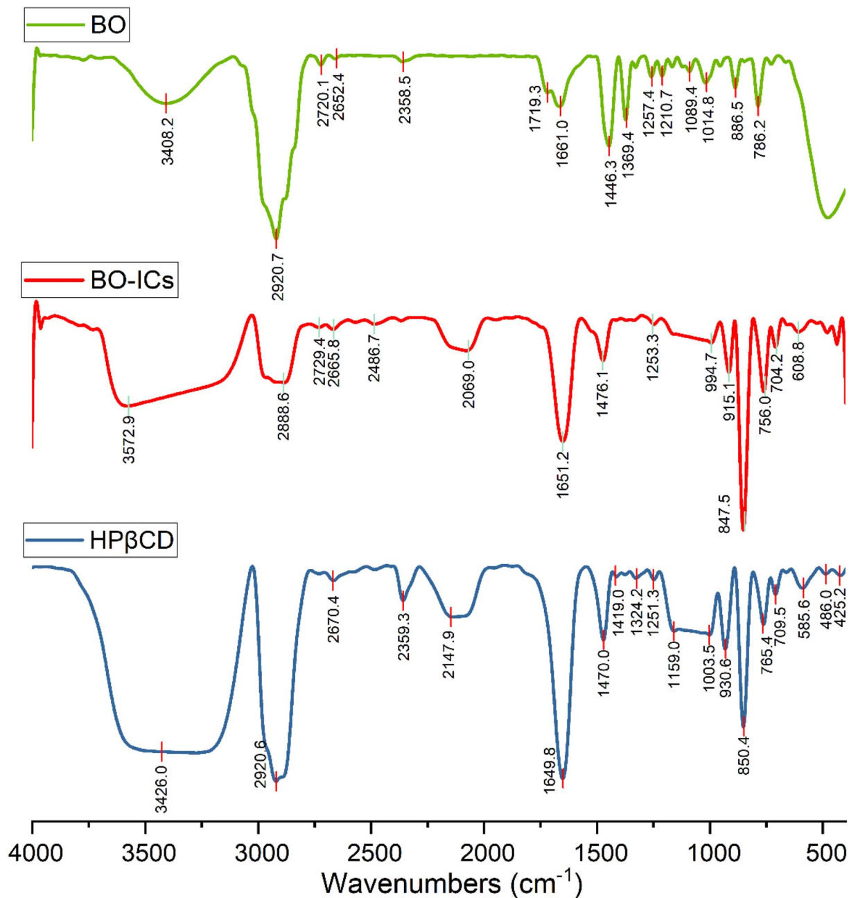
Fig. 3 FTIR spectra of BO, BO-ICs, and HP \beta CD.
