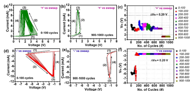
Fig. 3 Sweep bias polarity dependent electrical transport measurements of the vanadium oxide crystalline sample. (a) Discrete threshold switching over the initial 0 – 100 I – V cycles during positive sweep. (b) Switching between 900 – 1000 cycles. (c) Distribution of V_{\text{th}} voltages vs. number of cycles with \Delta V_{\text{th}} of 0.20\text{ V} . (d) Discrete switching in negative sweep for the initial 0 – 100 cycles. (e) Switching between 900 – 1000 cycles. (f) Distribution of V_{\text{th}} voltages vs. number of cycles with \Delta V_{\text{th}} of 0.20\text{ V} .
