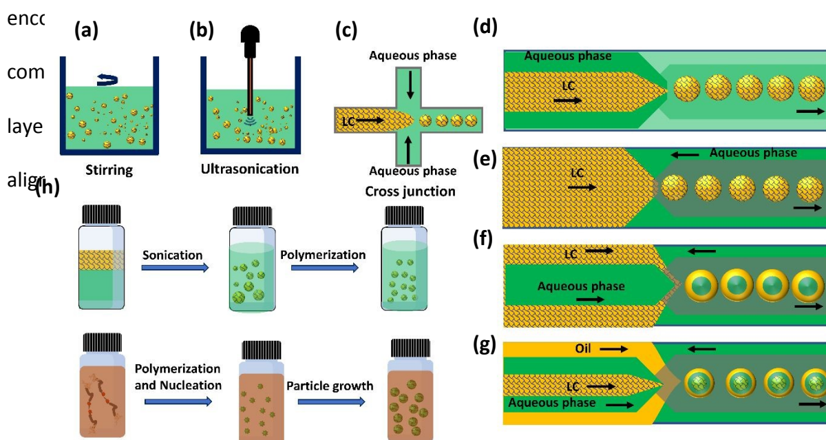
Figure 3. Schematics depicting the production process of LC emulsions: Emulsification through (a) stirring, (b) ultrasonication represent bulk emulsification strategies. Microfluidic emulsification using (c) PDMS cross-junction microchannel, while (d-g) involve microfluidic emulsification using a tip-to-tip microchannel, enabling the fabrication of single emulsion (d&e), double emulsion(f), and triple emulsion(g), respectively. (h). suspension (top)and precipitate polymerization (bottom)
