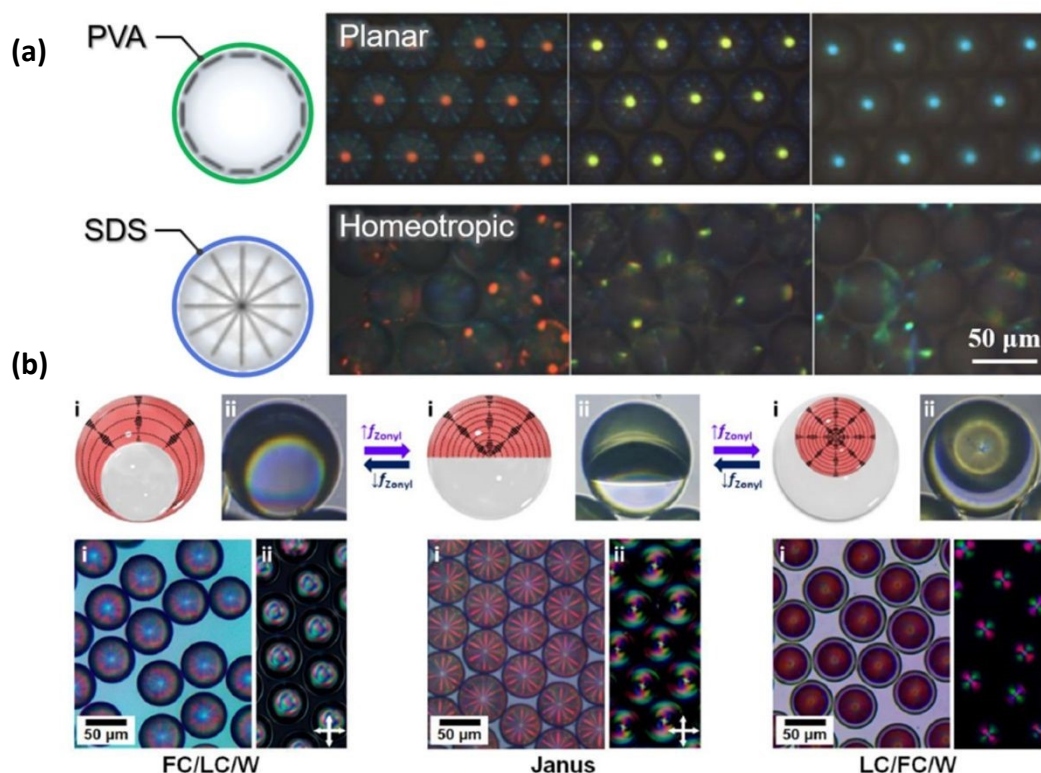
Figure 4. (a) Cholesteric LC droplets exhibiting planar and homeotropic configuration. Adapted from Ref. 74 with permission. Copyright © 2016 American Chemical Society. (b). Complex LC emulsions exhibiting dynamic reconfiguration in response to variations in surfactant content between F/LC/W double emulsions, Janus droplets, and LC/F/W double emulsions. Adapted with permission from Ref. 77
