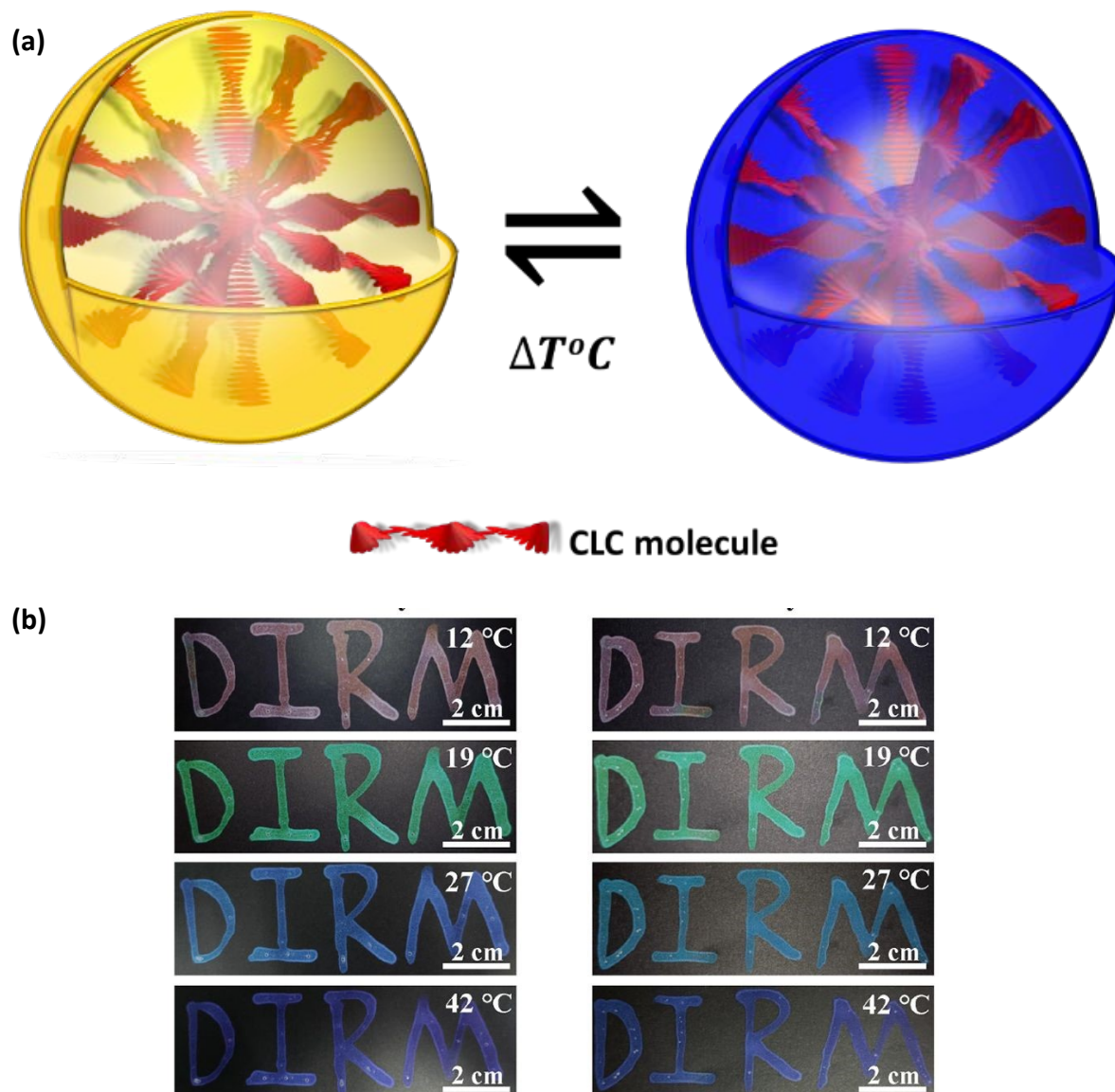
Figure 6 (a). Principle of anticounterfeiting using temperature as stimuli (b). Thermochromic coatings of cholesteric LC microcapsules with cellulose nanocrystals (CNC) and a melamine-formaldehyde (MF) resin hybrid shell with and without dye. Adapted from Ref. 85 with permission. Copyright © 2022 American Chemical Society.
