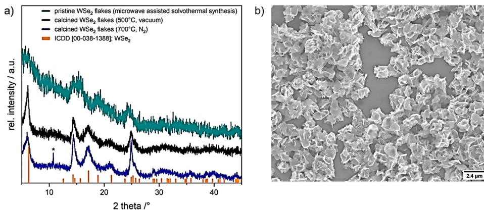
Fig. 3 (a) XRD patterns of microwave assisted solvothermal decomposition of [W\{(SeC_2H_4)_2NMe\}_2] precursor in NMP (cyan) and calcined WSe_2 flakes (500 °C, vacuum) (black) and under nitrogen atmosphere at 700 °C (for 7 h) (blue), reference WSe_2 (ICDD 00-038-1388) is shown in orange, *showing a peak which could assume the formation of WO_2 (ICDD 00-082-0728, WO_2 ; Fig. S5, ESI†). (b) SEM micrograph of resulting WSe_2 microstructures.
