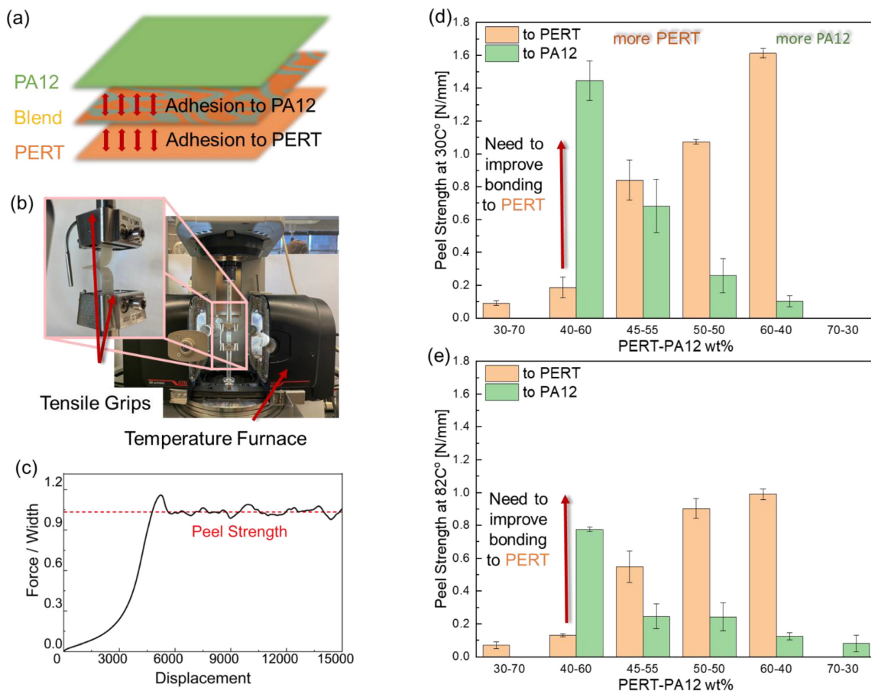
Fig. 1 T-peel test setup and measured peel strength of PERT-PA12 blends to PERT and PA12. (a) Schematic of Trilayer sample, which uses an immiscible blend as an adhesion layer to bond the two dissimilar layers. (b) T-peel test setup consisting of tensile grips and temperature furnace. (c) Example of force/width vs. displacement curve and peel strength at the steady-state plateau. Peel strength of PERT-PA12 to PERT and PA12 at (d) 30 °C, and (e) 82 °C.
