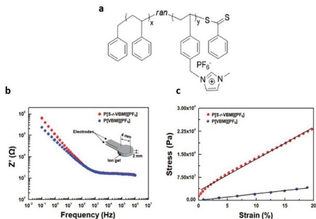
Fig. 26 (a) Schematic representation of the random copolymer-based ionic conductive gel. (b) Resistance ( Z' ) versus frequency (Hz) plots and (c) stress-strain curves for the ion gels composed of 40 wt% P[S-r-VBMI][PF 6 ] or P[VBMI][PF 6 ] and 60 wt% [EMIM][TFSI]. The inset of (b) depicts the electrode/ion gel/electrode cell structure used in electrochemical impedance spectroscopy (EIS) experiments. Reproduced from ref. 4 with permission from Wiley-VCH, Copyright [2018].
