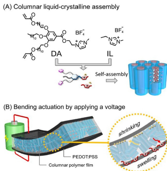
Fig. 15 (A) Molecular structures of the wedge-shaped imidazolium compound with diacrylate groups (DA) and ionic liquid [EMIM][BF 4 ] (IL) and their self-assembly into the columnar liquid-crystalline phase forming 1D ion channels. (B) Illustration of the electric-field-driven bending actuation of the three-layer membranes composed of the columnar liquid crystalline polymer electrolyte and PEDOT:PSS electrodes. Reproduced from ref. 107 with permission from ACS, Copyright [2022].
