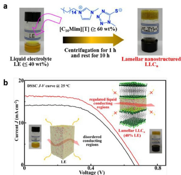
Fig. 17 (a) Preparation of LLCn from organic LE and [C 16 Mim][T]. (b) Schematic representation of lyotropic liquid crystals inducing liquid-fluid lamellar conducting highways. Reproduced from ref. 109 with permission from ACS, Copyright [2022].
