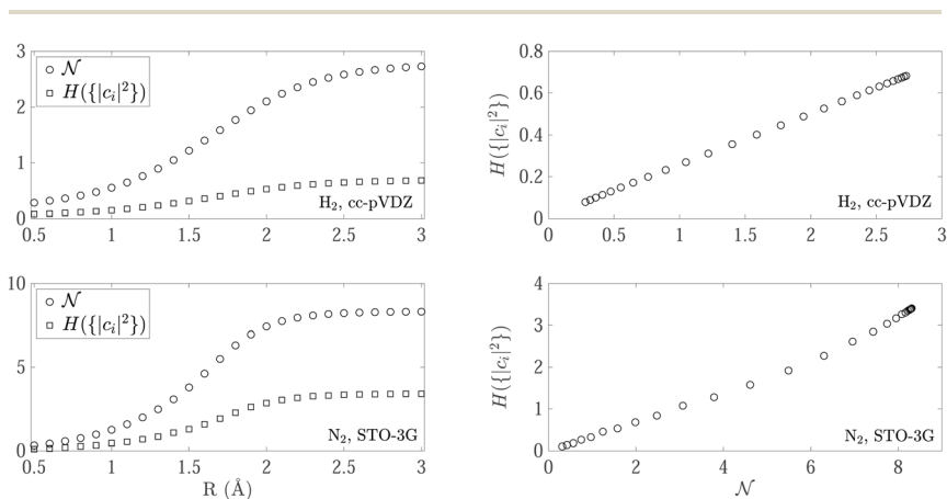
Fig. 7 Nonfreeness \mathcal{N} and Shannon entropy H(\{|c_i|^2\}) of the CI expansion coefficients in natural orbital basis for the full CI ground state of \text{N}_2 in the STO-3G basis at various internuclear distances R (left), and H(\{|c_i|^2\}) as a function of \mathcal{N} (right).
