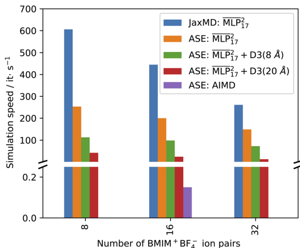
Fig. 2 Inference times of the original and hybrid \overline{\text{MLP}}^2_{17} + \text{D3} models for different system sizes on a single RTX 4090 GPU compared to AIMD simulations on 256 cores.
