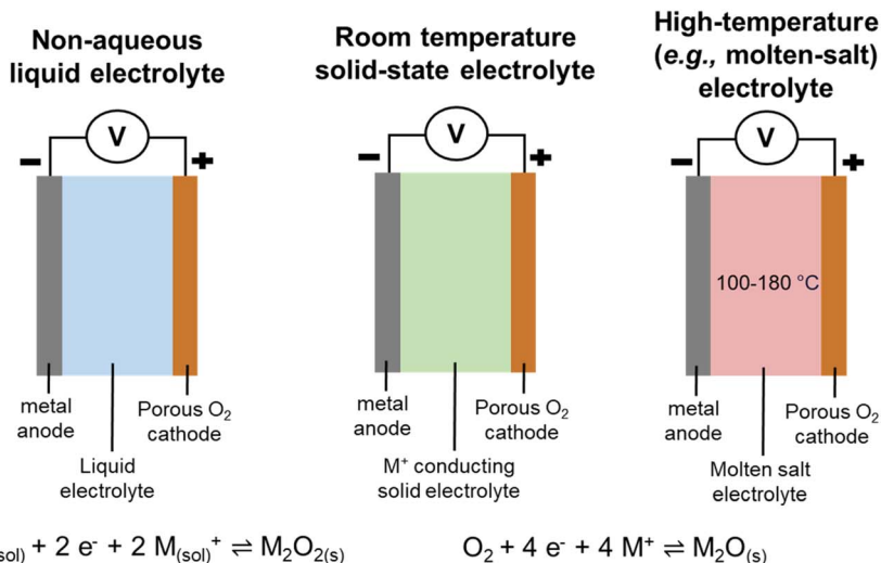
Fig. 2 Various configurations of (open) alkali-metal–O 2 cell chemistries.
