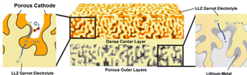
Fig. 4 Concept of a tri-layer garnet \text{Li}_7\text{La}_3\text{Zr}_2\text{O}_{12} (LLZ) Li–O 2 cell with high interfacial surface area, short lithium-ion conduction pathways and minimized use of electrolyte material, taken from https://doi.org/10.1039/D3FD00119A .
