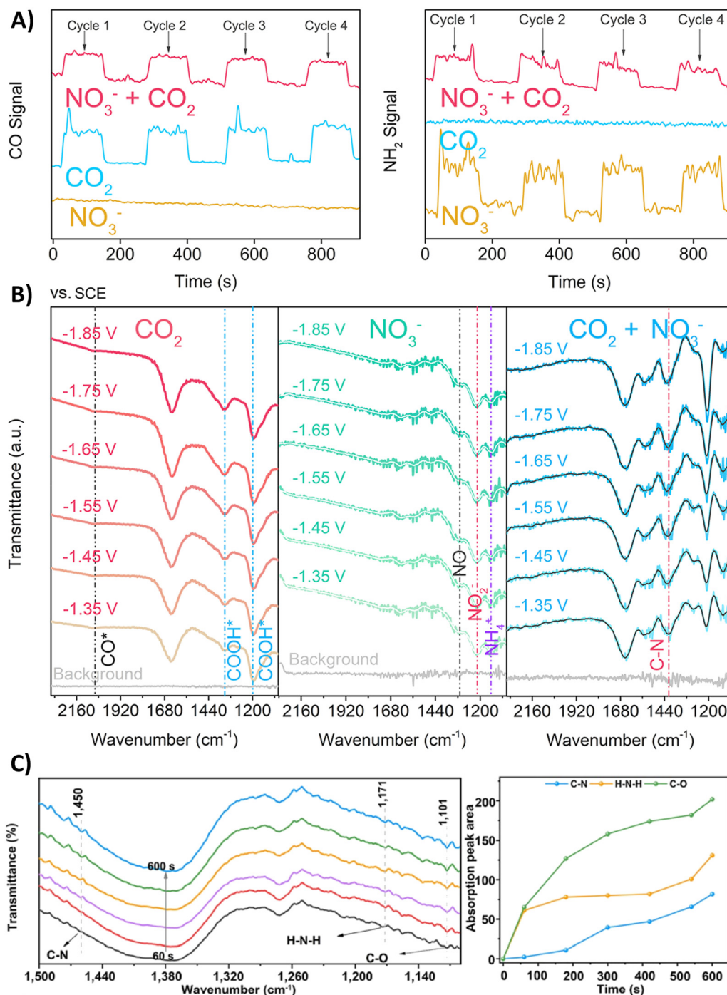
Fig. 13 Mechanistic investigations involving the formation of ^*\text{H}_2\text{NCO} . (A) Online DEMS spectra of CO and \text{NH}_2 signals over Cu@Zn catalyst in mixtures containing \text{CO}_2 , \text{NO}_3^- or \text{CO}_2 + \text{NO}_3^- . (B) In situ ATR-FTIR spectra of \text{CO}_2 , \text{NO}_3^- and mixture of \text{CO}_2 + \text{NO}_3^- electroreduction over Cu@Zn catalyst over different potentials. (C) In situ ATR-FTIR spectra as a function of electrolysis time for CoPc-COF@TiO 2 NTs catalyst and the intensity of the signals for C–O, H–N–H and C–N stretching vibrations as a function of electrolysis time. Adapted from ref. 176 (A) and (B) and 181 (C).
