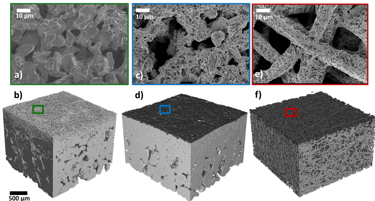
Fig. 3 (a), (c) and (e) Top view SEM images and (b), (d) and (f) XTM surface renderings of (a) and (b) MPL + support layer; (c) and (d) MPE with 2.5 \text{ mgIr cm}^{-2} loading; and (e) and (f) Ti-felt (Bekaert) with 2.5 \text{ mgIr cm}^{-2} .
