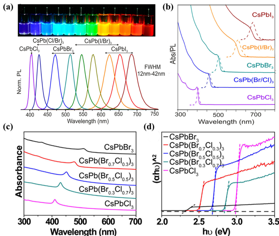
Fig. 4 (a) Colloidal halide perovskite \text{CsPbX}_3 NCs ( \text{X} = \text{Cl}, \text{Br}, \text{and I} ) exhibit size- and composition-tunable bandgap energies covering the entire visible spectral region with narrow and bright emission. 64 (b) Typical optical absorption and PL spectra of \text{CsPbX}_3 NCs. 64 (c) UV-vis absorption spectra and (d) (\alpha h\nu)^2 versus h\nu curves of \text{CsPb}(\text{Br}_x/\text{Cl}_{1-x})_3 ( x = 1, 0.7, 0.5, 0.3, 0 ) materials. 65
