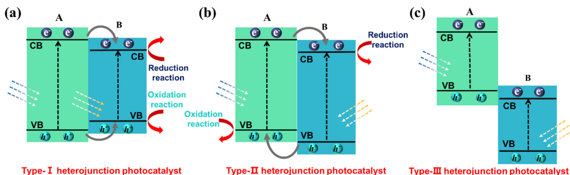
Fig. 14 Schematic illustration of electron-hole separation of three conventional heterojunctions: (a) type-I, (b) type-II and (c) type-III.
