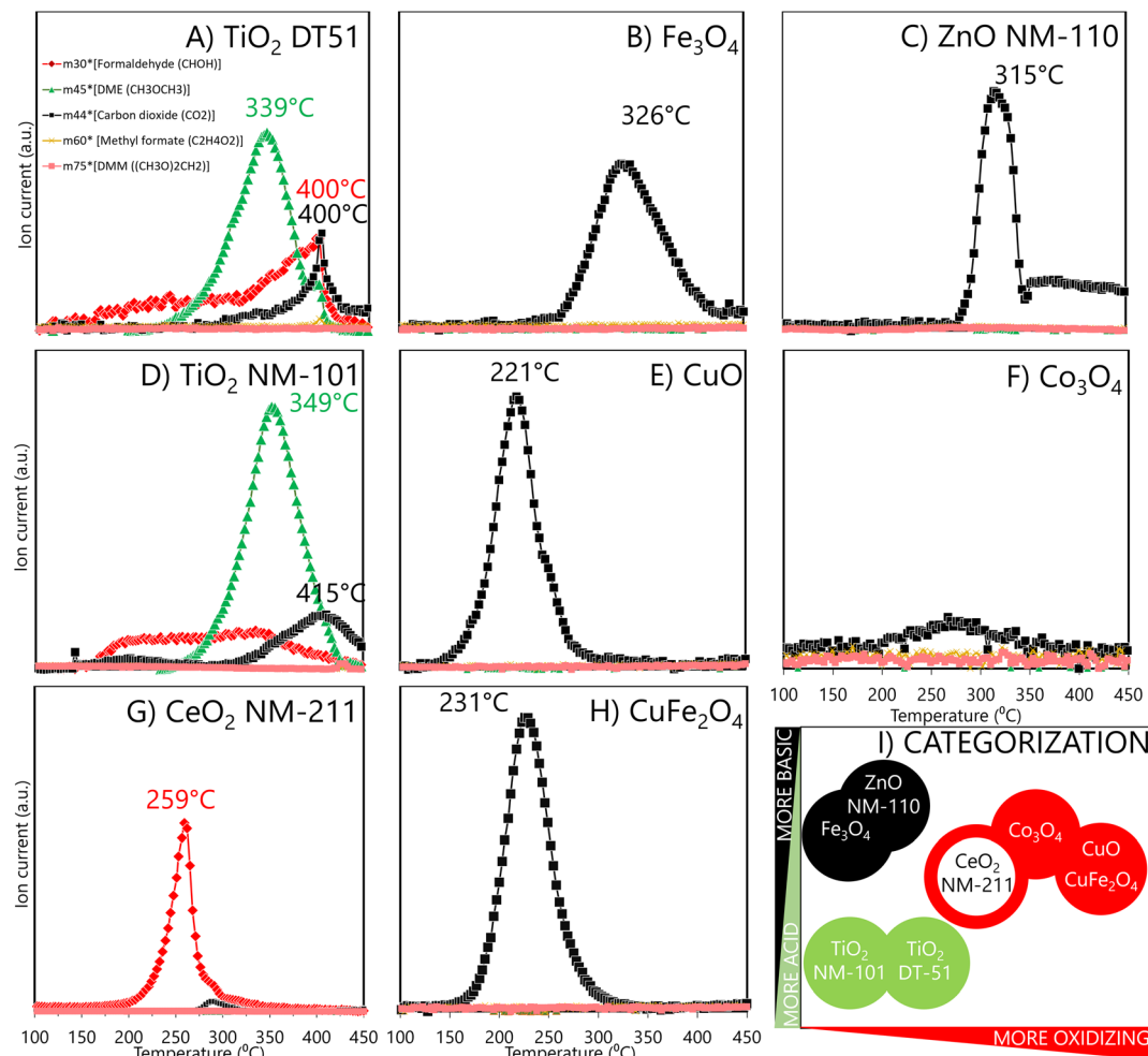
Fig. 3 Temperature-programmed surface reaction products of pre-adsorbed methanol analysed by mass spectroscopy for two different anatase TiO 2 : DT51 (A) and NM-101 (D), for Fe 3 O 4 -SA (B), for ZnO NM-110 (C), for CuO-SA (E), for Co 3 O 4 -SA (F) for CeO 2 NM-211 (G), and for CuFe 2 O 4 -SA (H). Formaldehyde signal (red) is obtained for redox sites, a dimethyl ether signal (green) for acid sites, and carbon dioxide (black) for basic or high reactive redox sites. ENM classification by MeOH-TPSR results is shown in I) with the same colour code. For a given colour, filled circles are more reactive than empty circles.
