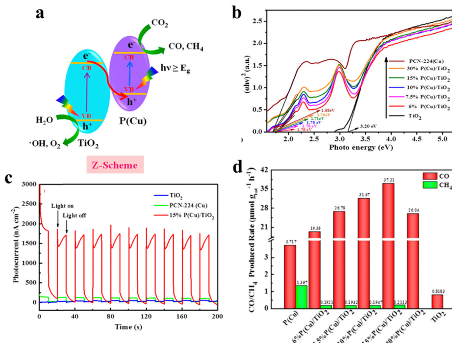
Fig. 14 (a) Direct Z-scheme photocatalytic mechanism. (b) Energy band gaps ( E_g ) of TiO 2 , PCN-224(Cu), and PCN-224(Cu)/TiO 2 . (c) Photocurrent–time ( I – t ) curves of TiO 2 , PCN-224(Cu), and 15%P(Cu)/TiO 2 photoelectrodes at 0.6 V vs. REH bias potential in 0.5 M Na 2 SO 4 (pH ~7.35). (d) CO and CH 4 generation rate over PCN-224(Cu), 6%P(Cu)/TiO 2 , 7.5%P(Cu)/TiO 2 , 10%P(Cu)/TiO 2 , 15%P(Cu)/TiO 2 , 30%P(Cu)/TiO 2 , and TiO 2 under 300 W Xe lamps. Reproduced from ref. 64. Copyright 2022 ACS.
