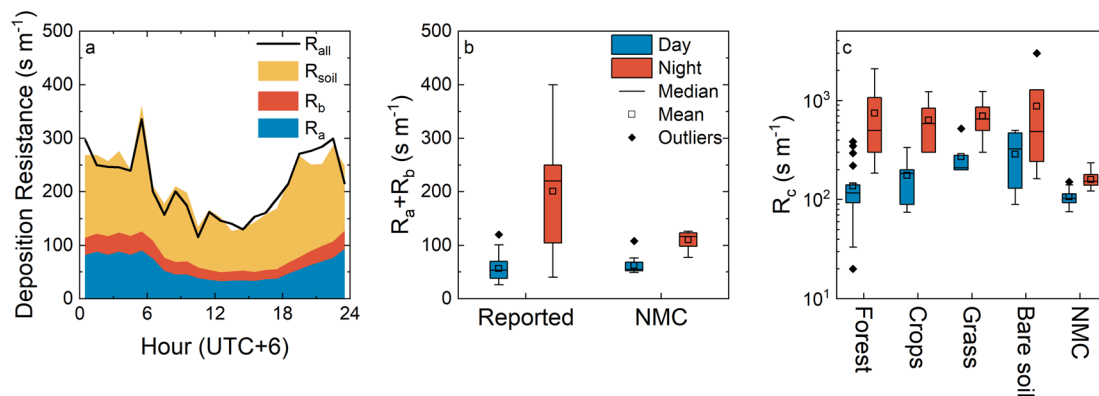
Fig. 3 (a) Median diel pattern of deposition resistance of observation at NMC site. Hourly medians are utilized instead of hourly means due to the skewed distribution of R_{all} and R_{soil} . (b) Comparison of R_a + R_b and reported R_a + R_b during day and night. (c) Comparison of observed R_{soil} and reported R_c over different conditions during day and night. Parts of reported R_c are obtained by 1/v_d minus prescribed R_a + R_b (50 s m -1 during daytime and 200 s m -1 during nighttime). Data from: 24,26,58–67
