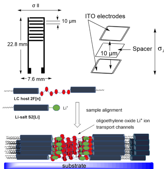
Fig. 6 Schematic representation of the electrodes and electrolyte. Top: interdigitated gold electrode and ITO cell. Bottom: parallelly aligned electrolyte sample inside the cell with oligo(ethylene oxide) channels for \text{Li}^+ ion transport.
