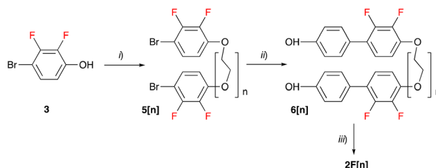
Scheme 1 Preparation of LC hosts 2F[n] . Reagents and conditions: (i) t -BuOK, EtOH, \text{Ts}(\text{OCH}_2\text{CH}_2)_n\text{OTs} ( 4[n] ), reflux, 18 h, and 69–90% yield; (ii) 4- \text{OHC}_6\text{H}_4\text{B}(\text{OH})_2 , \text{Pd}_2(\text{dba})_3 , [\text{HPCy}_3][\text{BF}_4] , t -BuOK, THF/ \text{H}_2\text{O} , reflux, 48 h, and 61–74% yield; (iii) 4-hexylbenzoic acid, EDC-HCl, DMAP, \text{CH}_2\text{Cl}_2 , rt, 18 h, and 60–78% yield.
