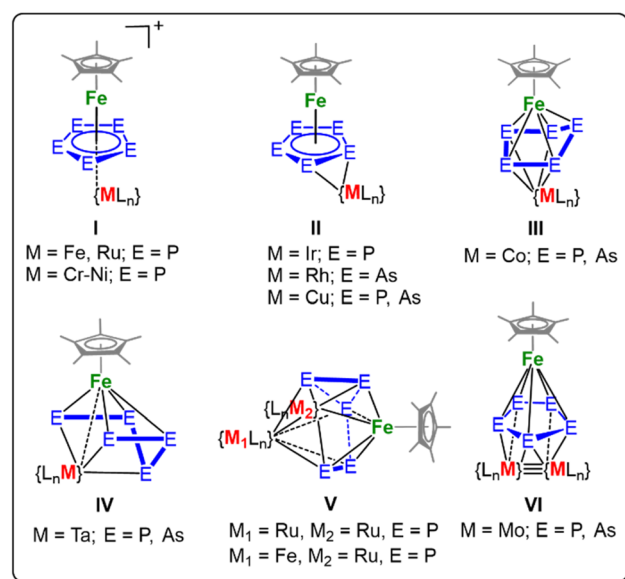
Fig. 1 Selected examples reported for heterometallic polypnictogen complexes containing \text{E}_5 ligands derived from 1 and 2 , respectively. (I: \{\text{ML}_n\} = \{\text{Cp}^*\text{Fe}\}, \{\text{Cp}^*\text{Ru}\}, \{\text{Cp}^*\text{Ru}\}, \{\text{Cp}^*\text{Cr}\}, \{\text{Cp}^*\text{Mn}\}, \{\text{Cp}^*\text{Fe}\}, \{\text{Cp}^*\text{Co}\}, \{\text{Cp}^*\text{Ni}\} ; II: \{\text{ML}_n\} = \{\text{Cp}^*\text{Ir}(\text{CO})\}, \{\text{Cp}^*\text{Rh}(\text{CO})\}, \{\text{nacnacCu}\} ; III: \{\text{ML}_n\} = \{\text{Cp}^*\text{Co}\} ; IV: \{\text{ML}_n\} = \{\text{Cp}^*\text{Ta}\} ; V: \{\text{ML}_n\} = \{\text{Cp}^*\text{Ru}\}, \{\text{Cp}^*\text{Fe}\} ; VI: \{\text{ML}_n\}_2 = \text{Mo}_2[\mu_2\kappa^2\text{-Me}_2\text{Si}(\text{N-2,6-iPr}_2\text{C}_6\text{H}_3)_2]_2 ; \text{Cp}^* = 1,3\text{-tBu}_2\text{C}_5\text{H}_3 , \text{Cp}^{**} = 1,2,4\text{-tBu}_3\text{C}_5\text{H}_2 , \text{Cp}^* = \text{C}_5\text{Me}_5 , \text{nacnac} = \{\text{N}(\text{C}_6\text{H}_3\text{Me-2,6})\text{CMe}_2\text{CH} .
