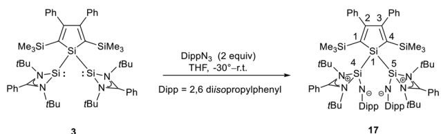
Scheme 3 Reaction of bis(silylene)silole 3 with 2,6-diisopropylphenylazide.
