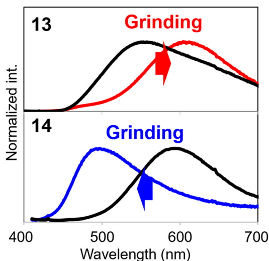
Fig. 6 Mechanochromic luminescence and self-recovery of 13 and 14 . Reprinted with permission from ref. 34. Copyright 2023 Wiley-VCH Verlag GmbH & Co. KGaA, Weinheim.
