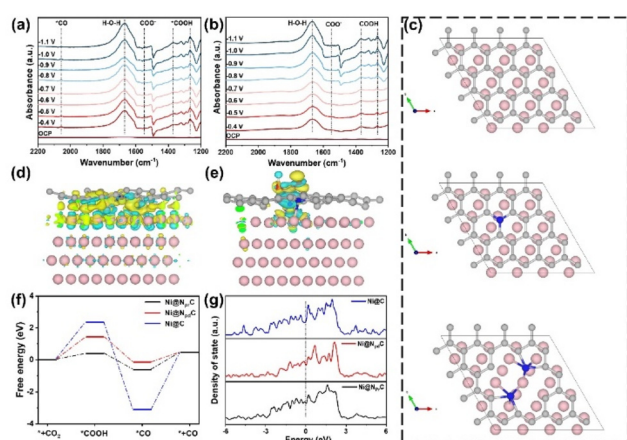
Fig. 5 The in situ FTIR spectra of (a) Ni@NC-1000 and (b) NC-1000. (c) The models of Ni@C, Ni@N pd C and Ni@N pr C. The charge density distribution on Ni@N pr C before (d) and after (e) *COOH intermediate sorption (the yellow and cyan areas represent electron accumulation and depletion). (f) The free-energy diagram for the CO 2 RR to CO on Ni@C, Ni@N pd C and Ni@N pr C. (g) The density of states for Ni@C, Ni@N pd C and Ni@N pr C.
