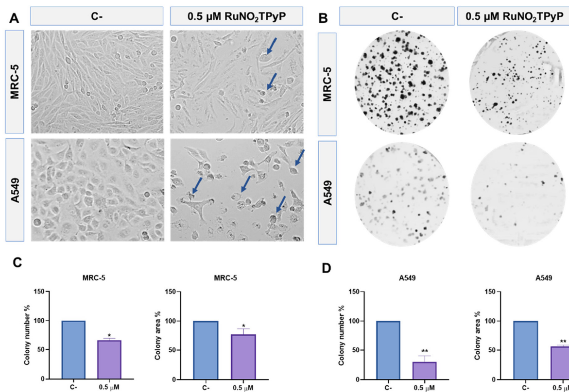
Fig. 3 Effects of RuNO 2 TPyP on MRC-5 and A549 after 4 h of treatment (0.5 \mu M) followed by irradiation at 415 nm (4 J cm -2 ) on (A) cell morphology, arrows indicate drastic alterations in morphology; (B) colony formation; and (C) quantitative analysis of MRC-5 colony numbers and area (D) quantitative analysis of A549 colony number and area (* p < 0.05 and ** p < 0.01).
