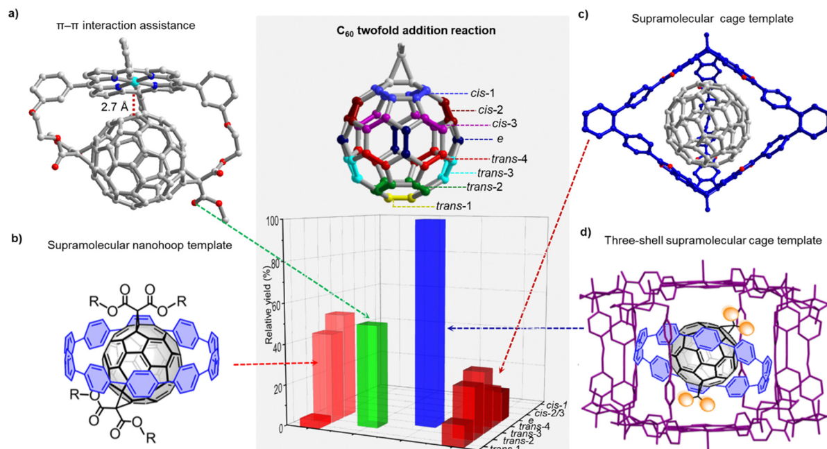
Fig. 3 Selected methods for regioselective twofold addition reactions to C 60 . (a) \pi - \pi interaction assistance. (b) Supramolecular nanohoop template. (c) Supramolecular cage template, 3 equiv. N -methylglycine was used. (d) Three-shell supramolecular mask strategy.
