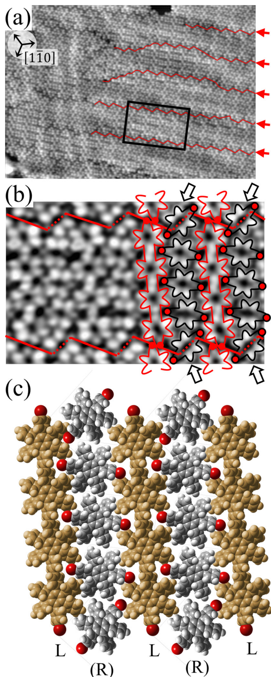
Fig. 3 (a) STM image ( 40 \text{ nm} \times 30 \text{ nm} , V_s = -3.0 \text{ V} , and I_t = 20 \text{ pA} ) of \text{Br}_2 -HPB covered Au(111) after annealing at 200 \text{ }^\circ\text{C} for 1 h. The periodic zigzag dark lines are observed, indicated by red lines and red arrows. Typically, the zigzag dark lines run parallel to 0^\circ or \pm 20^\circ deviated from the [1\bar{1}0] direction of the underlying Au(111) surface. (b) Enlarged STM image ( 10 \text{ nm} \times 5 \text{ nm} ) of the region indicated by the black rectangle in (a). The zigzag row is composed of periodically arranged HPB polymer chains and \text{Br}_2 -HPB molecules, depicted by red and black outlines on the right, respectively. (c) Expected self-assembled structure of the mixture phase for (b), in which the L-type HPB polymers are represented by brown, and the chiral-unidentified \text{Br}_2 -HPB molecules are represented by grey, respectively. For the minimized intermolecular steric hindrance, the heterochiral arrangement of homochiral rows are expected.
