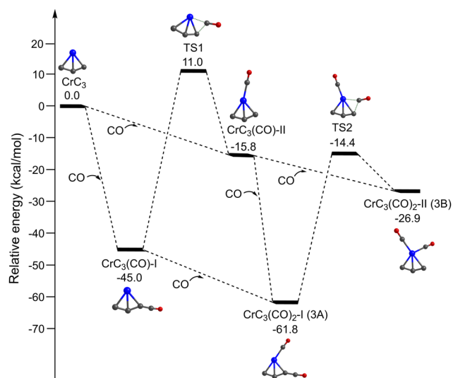
Fig. 4 Potential energy profiles of the CrC _3 + 2\text{CO} \rightarrow \text{CrC}_3(\text{CO})_2 reaction calculated at the B2PLYPD3//BLYP-D3(BJ)/def2-TZVPP level of theory. Energies are given in kcal mol ^{-1} . All the molecules are in a quintet state.
