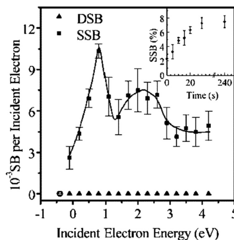
Fig. 22 Yield of single strand breaks (squares) as a function of electron kinetic energy. Reproduced from Fig. 11 in ref. 75 with permission from the American Chemical Society (2006).
