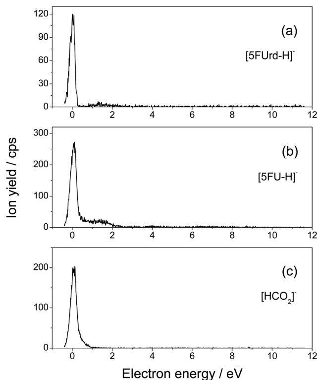
Fig. 2 Yield function of the (a) dehydrogenated parent anion [5\text{FUr-H}]^- , (b) dehydrogenated 5-fluorouracil anion [5\text{FU-H}]^- produced from the N -glycosidic bond cleavage, and (c) [\text{HCO}_2]^- anion.
