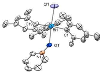
Fig. 5 Solid state structure of 13 . Ellipsoids are drawn at the 50% probability level. H atoms and BaR f are omitted for clarity. Selected bond lengths (Å) and angles (°): Bi1–Cl1: 2.507(7), Bi1–O1: 2.404(6), Bi1–C1: 2.229(6), Bi1–C10: 2.226(5), Bi1–C19: 2.236(6), N1–O1: 1.334(8), C1–Bi1–C10: 117.9(2), C1–Bi1–C19: 121.7(2), C10–Bi1–C19: 119.3(2), Cl1–Bi1–O1: 173.5(2), N1–O1–Bi: 136.7(4).
