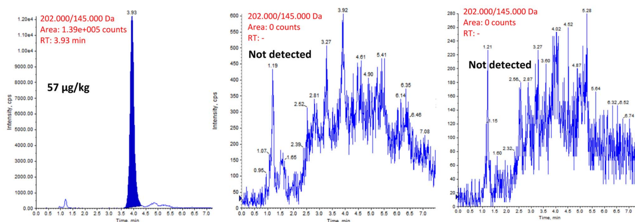
Fig. 2 LC-MS/MS chromatogram of (a) isoprocarb and (b) carbaryl in contaminated robusta coffee during coffee processing.
