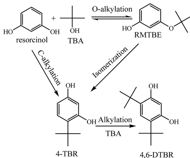
Scheme 3 The possible reaction mechanism for t -butylation.
