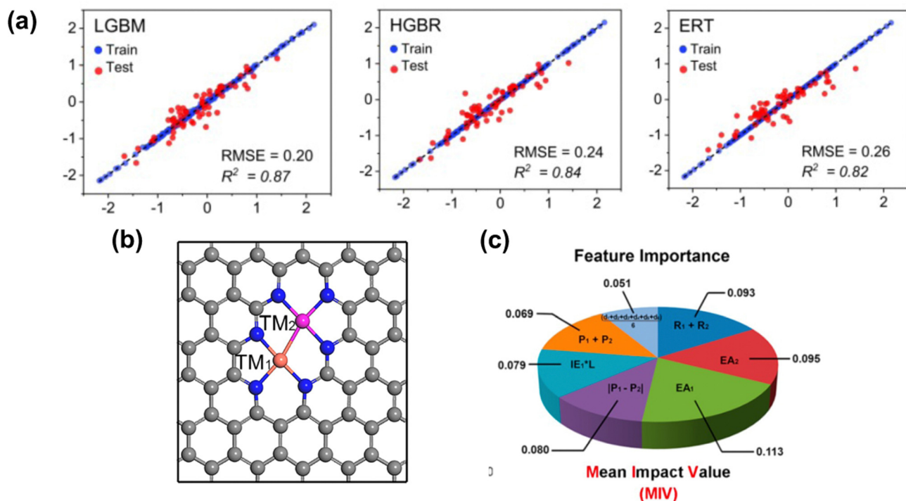
Fig. 4 (a) Machine learning model performance for predicting the adsorption energy of \text{H}^\ast on 2D carbon materials. (b) Schematic illustration of the bi-metal site on graphene. (c) Mean impact value (MIV) employed for considering feature importance. Reprinted with permission from ref. 159. Copyright 2022 Royal Society of Chemistry.
