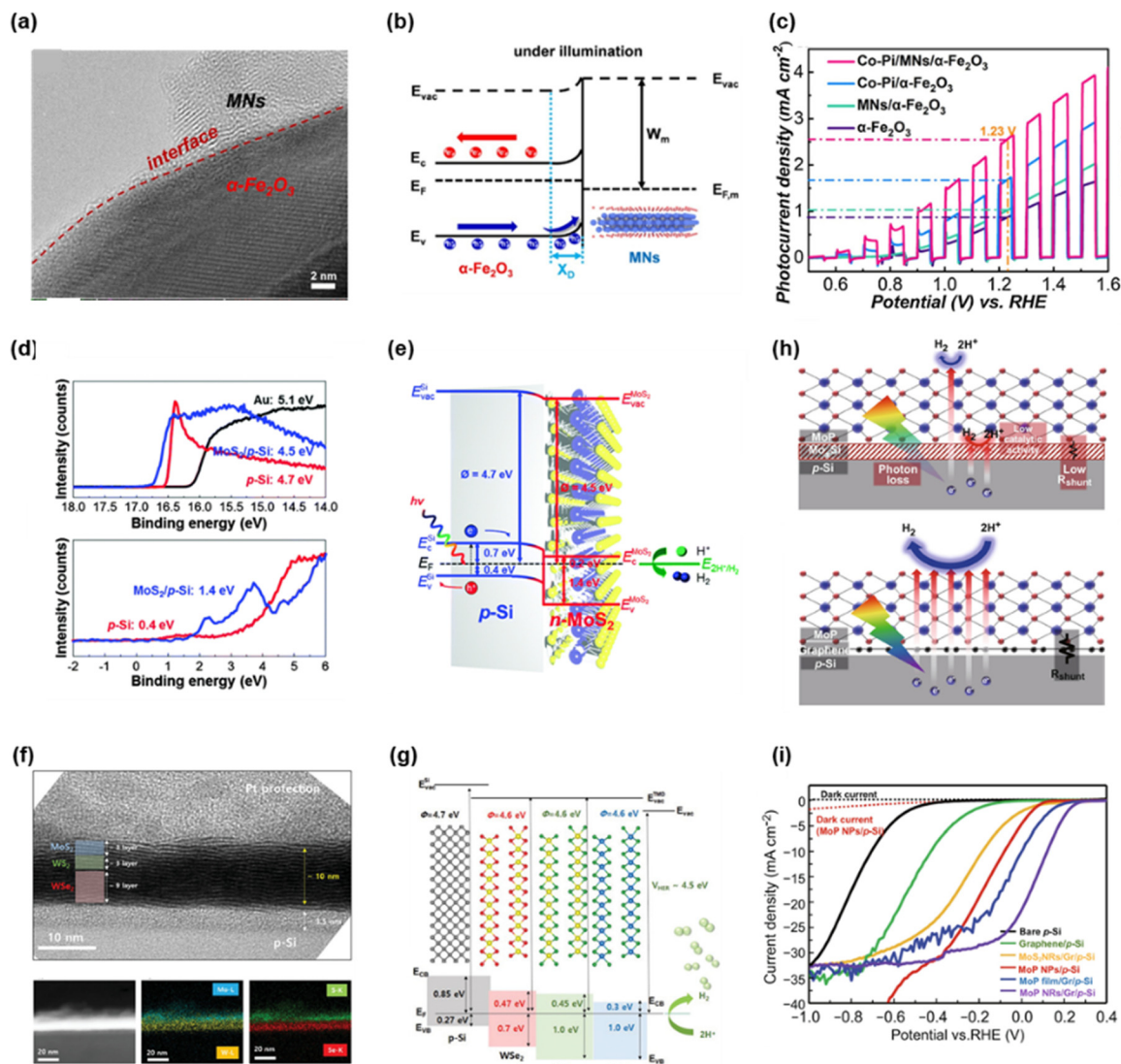
Fig. 3 (a) High-resolution TEM image of MXene nanosheets/ \alpha -Fe 2 O 3 . (b) Energy band diagram of MXene nanosheets/ \alpha -Fe 2 O 3 Schottky junction under illumination. (c) LSV curves of \alpha -Fe 2 O 3 , MNs/ \alpha -Fe 2 O 3 , Co-Pi/ \alpha -Fe 2 O 3 , and Co-Pi/MNs/ \alpha -Fe 2 O 3 . Copyright 2021, Elsevier. (d) UPS and XPS spectra of Au, p-Si, and MoS 2 /p-Si. (e) Schematic of energy band diagram of the MoS 2 /p-Si photocathode having p-n junction. Copyright 2016, Royal Society of Chemistry. (f) Cross-sectional high-resolution TEM image for 112-MWW/p-Si thin film. Copyright 2019, Wiley-VCH GmbH. (g) Schematic of energy band diagram of 112-MWW/p-Si thin film. Copyright 2019, Wiley-VCH GmbH. (h) Schematic of MoP/Mo 3 Si/p-Si and MoP/graphene/p-Si. (i) LSV curves of bare p-Si, graphene/p-Si, MoS 2 NRs/Gr/p-Si, MoP NPs/p-Si, MoP film/Gr/p-Si, and MoP NRs/Gr/p-Si. Copyright 2021, Springer Nature.
