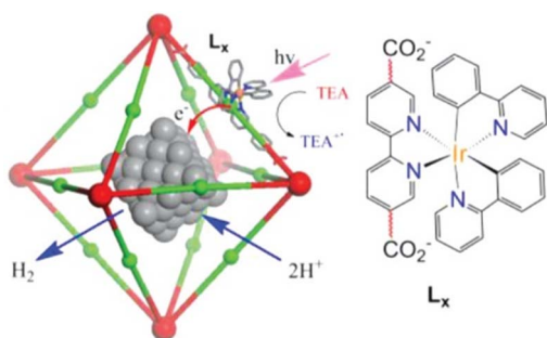
Fig. 3 Reaction scheme for the photocatalytic H 2 evolution via photoinjection of electrons from the light-harvesting MOFs into platinum NPs (PtNPs). The red and green balls represent Zr 6 (OH) 4 (-carboxylate) 12 cores and the Ir-phosphor ligand of the MOFs, respectively. Reprinted from ref. 73 with permission from American Chemical Society (Copyright 2012).
