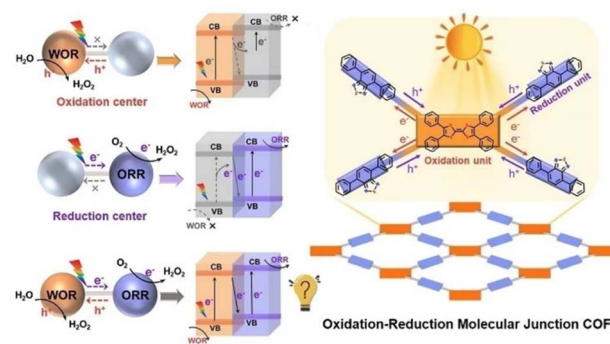
Scheme 12 Schematic diagram for \text{H}_2\text{O}_2 formation with a redox molecular-conjugated COF photocatalyst. Reprinted from ref. 99 with permission from John Wiley and Sons (Copyright 2023).
