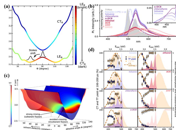
Fig. 6 (a) Potential energy surfaces of the \text{LE}_\text{B} and \text{CT}_\text{B} states along the torsional coordinate ( \Phi ) for dimer 12 . (b) Steady-state photoluminescence of dimer 12 in a range of solvents (solid lines). (c) Adiabatic potential energy surfaces along the dihedral angle \Phi and the solvent dielectric constant, showing their CT (blue) and TT (red) character. (d) Yield of long-lived CT (circles) and TT pairs (squares), extracted from excitation-dependent transient absorption measurements for solvents of increasing polarity (left to right). Reproduced with permission. 143 Copyright 2019, the American Chemical Society.
