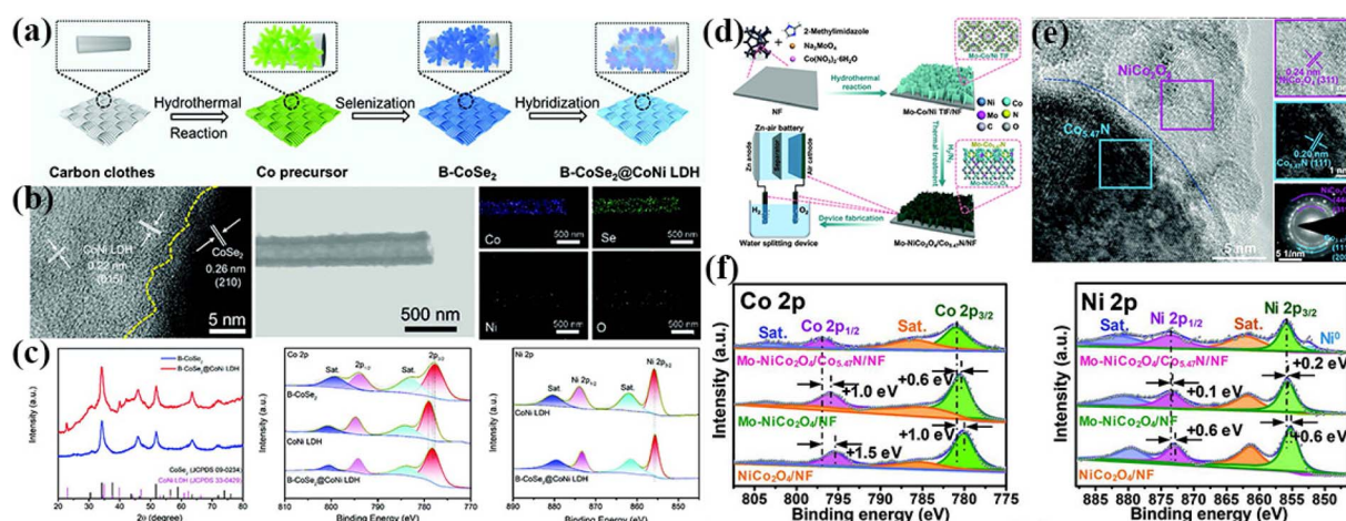
Fig. 7 (a) Schematic illustration of the synthetic process of B-CoSe 2 @CoNi LDH HNA. (b) HRTEM image of B-CoSe 2 @CoNi LDH HNA highlighting the interface between CoSe 2 and CoNi LDH and elemental mapping images of B-CoSe 2 @CoNi LDH HNA. (c) XRD spectra and XPS patterns for B-CoSe 2 , CoNi LDH, and B-CoSe 2 @CoNi LDH HNA. Reproduced with permission from ref. 152, Copyright (2022) Wiley. (d) Schematic illustration of the synthetic process of Mo–NiCo 2 O 4 /Co 5.47 N/NF. (e) HRTEM images and SAED pattern of Mo–NiCo 2 O 4 /Co 5.47 N/NF. (f) XPS spectra of Mo–NiCo 2 O 4 /Co 5.47 N/NF, Mo–NiCo 2 O 4 /NF, and NiCo 2 O 4 /NF. Reproduced with permission from ref. 154, Copyright (2020) Wiley.
