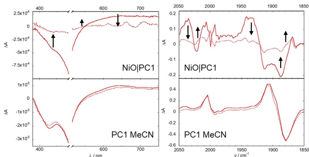
Fig. 3 UV-visible transient absorption spectra (left) and time resolved infrared spectra (right) for PC1 , 1 ps (solid line) and 1 ns (dotted line) following excitation at 500 nm in acetonitrile (bottom) and on a NiO thin film (top). The transient features at 1 ns spectrum for NiO|PC1 are imprints of the probe spectrum.
