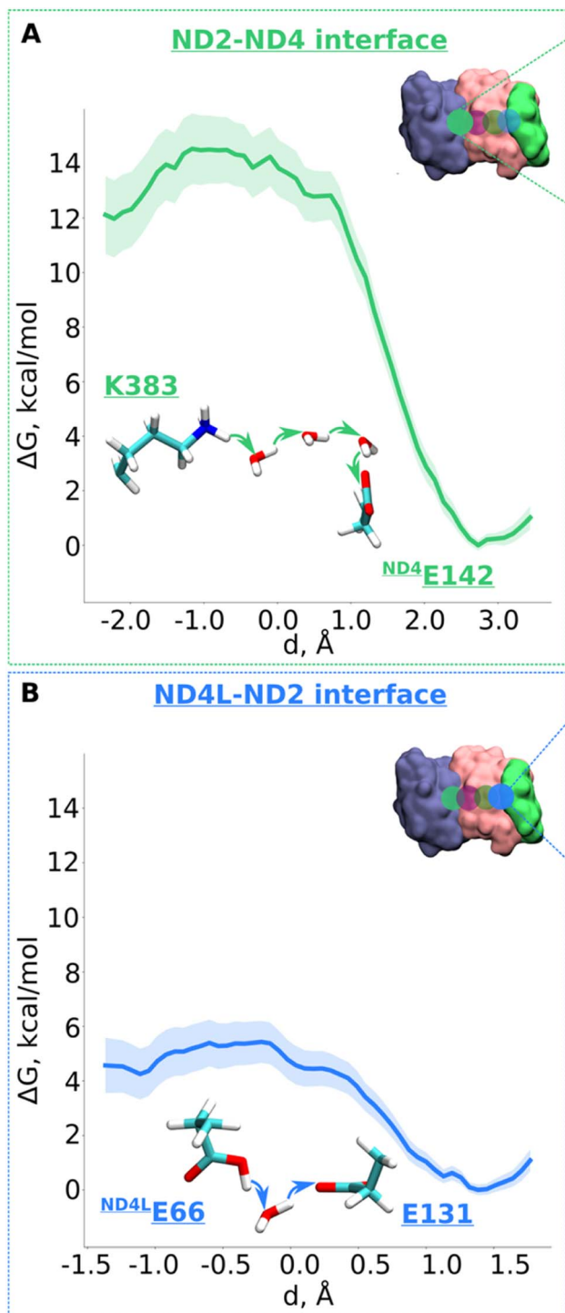
Fig. 5 Free energy profiles of the proton transfer in the “interface regions”. (A) ND2-ND4 interface: Lys383 (protonated) \rightarrow H 2 O \rightarrow H 2 O \rightarrow H 2 O \rightarrow ND 4 Gu142 (deprotonated) pathway. (B) ND4L-ND2 interface: ND 4 L-Glu66 (neutral) - H 2 O - Glu131 (deprotonated) pathway. The bold lines are PMF profiles with light shaded area highlighting the bootstrapping error range (see also methods). Occupational histograms for the reaction coordinates are given in ESI, Fig. S17G and H.† The inset depicts the core membrane subunits of respiratory complex I: ND4 (blue), ND2 (pink), and ND4L (green). The green (A) and blue (B) circles denotes the QM region where the proton transfer is investigated.
