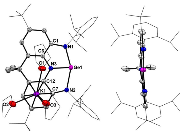
Fig. 3 Left: Solid-state structure of 4 . Right: Side view of the anionic part of 4 . The t\text{Bu} and Dipp groups are simplified as wireframes and hydrogen atoms are omitted for clarity. Thermal ellipsoids are set at the 30% probability level. Selected bond lengths (Å) and angles ( ^\circ ): \text{Ge1-N1} 2.0578(18), \text{Ge1-N2} 2.1633(18), \text{Ge1-N3} 1.9039(19), \text{C1-N1} 1.372(3), \text{C7-N2} 1.359(3), \text{C6-N3} 1.388(3), \text{C12-N3} 1.384(3), \text{C1-C6} 1.414(3), \text{C7-C12} 1.428(3), \text{N1-Ge1-N2} 153.81(7)^\circ , \text{N1-Ge1-N3} 78.23(7)^\circ , \text{N2-Ge1-N3} 76.56(7)^\circ .
