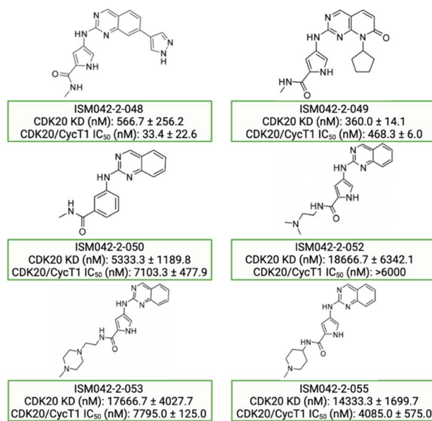
Fig. 7 Chemical structures for the second-round Chemistry42 generation for synthesis and testing in CDK20 binding and kinase activity assays. Biological data with a standard deviation are presented from three independent experiments.
