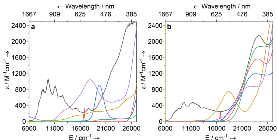
Fig. 3 UV-vis-NIR spectra of (a) 1-Ti and 2-M ( M = \text{Zr, La, Ce, Nd, U} ) and (b) 3-M ( M = \text{Ti, Zr, La, Ce, Nd, U} ) in toluene (2 mM) between 6000 and 27 000 \text{cm}^{-1} (1667–370 nm). Legend: M = \text{Ti} (yellow), \text{Zr} (purple), \text{La} (green), \text{Ce} (blue), \text{Nd} (red), \text{U} (black).
