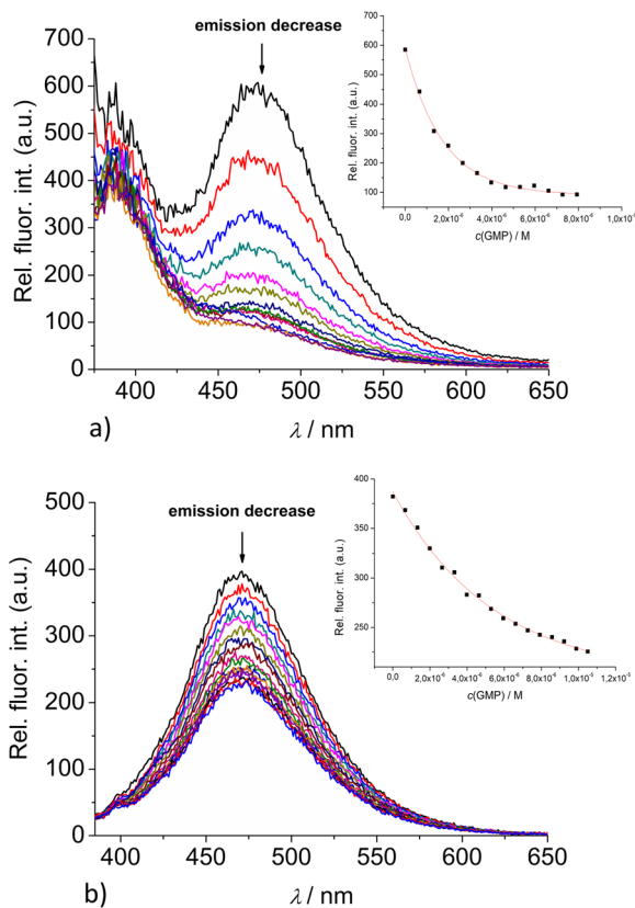
Fig. 4 Changes in the fluorescence spectra of: (a) 2 ( c = 5 \times 10^{-7} M) and (b) 3 ( c = 1 \times 10^{-6} M), upon titration with GMP ( c = 1 \times 10^{-5} M) at \lambda_{\text{exc}} = 350 nm. (Insets) Dependence of 2 and 3 emission intensity at 475 nm on c(\text{GMP}) . Done at pH 7.0, sodium cacodylate buffer, I = 0.05 M.
